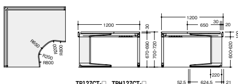
TR127CT-□ TRH127CT-□
