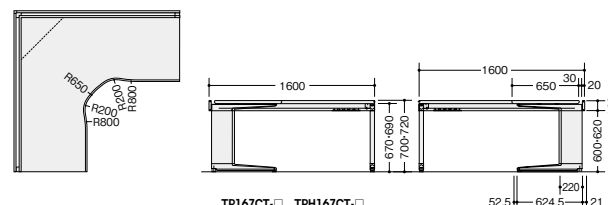
TR167CT-□ TRH167CT-□
