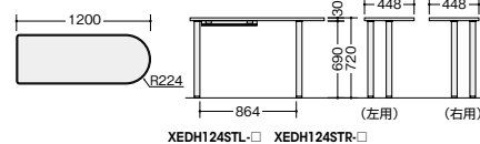
XEDH124STL-□ XEDH124STR-□
