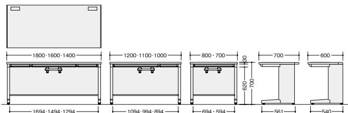
XED186F-□ XED166F-□ XED146F-□ XED126F-□ XED116F-□ XED106F-□ XED086F-□ XED187F-□ XED167F-□ XED147F-□ XED127F-□ XED117F-□ XED107F-□ XED087F-□ XED077F-□
