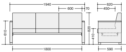
RC1223SF-□ RC1223S-□
