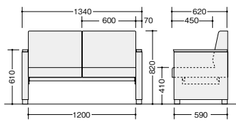
RC1222SF-□ RC1222S-□
