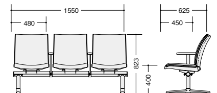
RC1353SHF-□ RC1353SH-□
