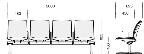
RC1354SHF-□ RC1354SH-□
