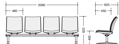
RC1354SF-□ RC1354S-□
