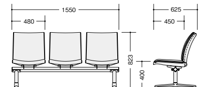
RC1353SF-□ RC1353S-□
