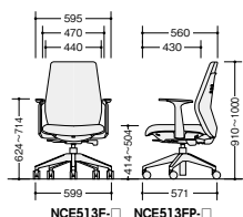
NCE513F-□ NCE513FP-□
