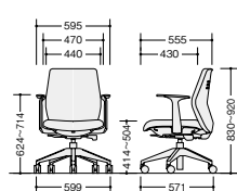
NCE511-□
