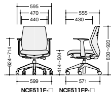
NCE511F-□ NCE511FP-□
