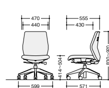
NCE510-□
