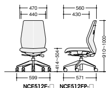
NCE512F-□ NCE512FP-□
