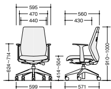
NCE513-□
