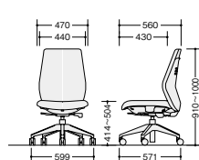
NCE512-□
