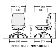
NCE510F-□ NCE510FP-□
