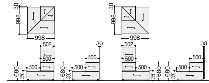
RC250EPR10-□ RC250EPL10-□
