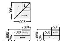
RC250E10-□
