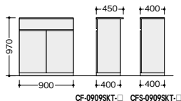
CF-0909SKT-□ CFS-0909SKT-□
