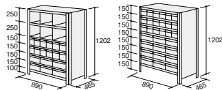
■F型引出し付棚 RLF435-04 ¥193,300
